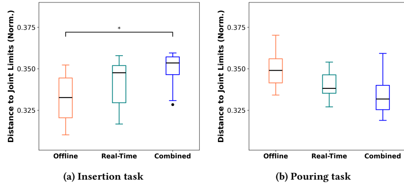
Figure 9: Distance to joint limits for both tasks: (a) insertion task and (b) pouring task.
