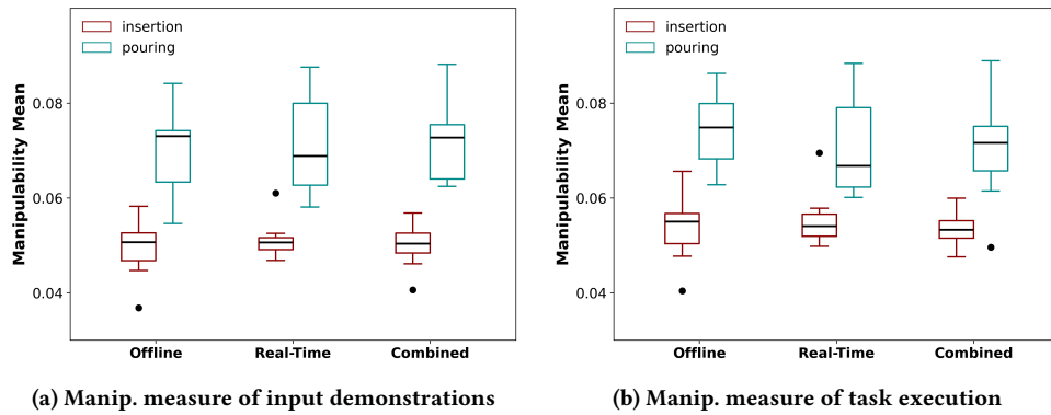
Figure 11: Manipulability measure of (a) input demonstrations and (b) robot task execution.
